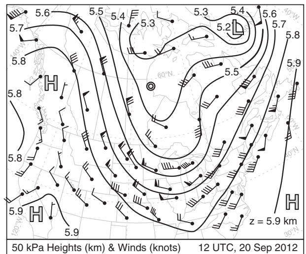
Figure 10.3 Winds ( 1\ knot \approx 0.5\ m\ s^{-1} ) and heights (km) on the 50 kPa isobaric surface. The relative maxima and minima are labeled as H (high heights) and L (low heights). Table 10-1 explains winds.
